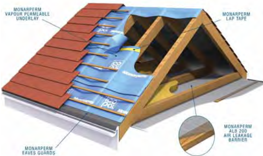
THE MONAPERM AIRTIGHT ROOF SYSTEM
